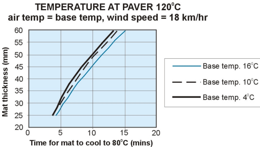
Figure 1: Cooling rate curves - Compaction of Asphalt Pavements, NCHRP: Synthesis of Highway Practice 152.
