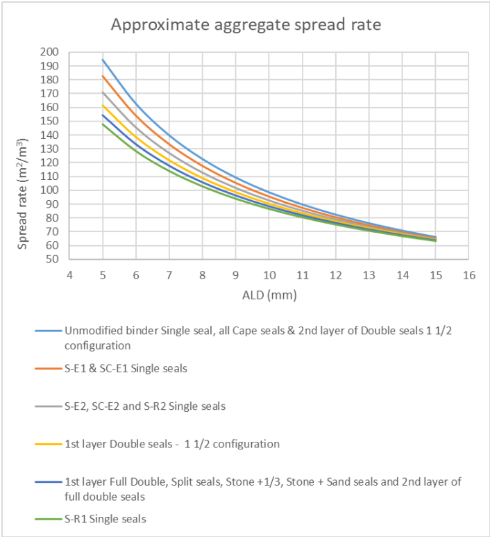
Figure F 27 Approximate Aggregate Spread Rates
