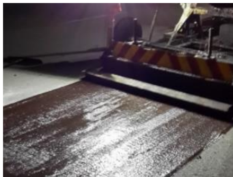
Figure F 11 Rut filling Without Concave Shape
