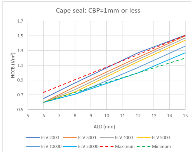
Figure E 34 Simulated Cape Seal Application Rates (Example)
