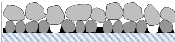
Figure C 11 Bridging of Large Aggregate Reseal
