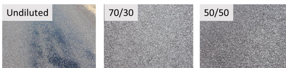
Figure H 21 Different Dilutions of Cationic Emulsions Applied
