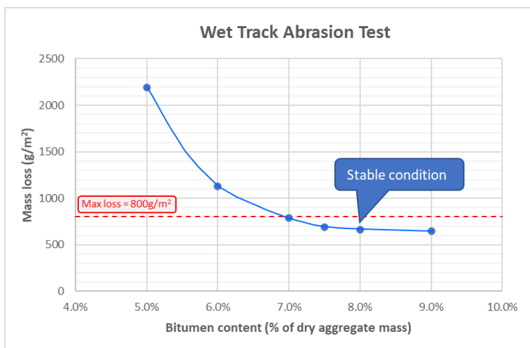
Figure E 45 Mass Loss versus Bitumen Content
