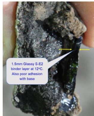
Figure C 28 S-E2 Binder Layer with Poor Adhesion to Base and Seal Aggregate
