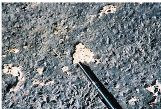
Figure F 39 Effect of Spraying Emulsion Before Cleaning
