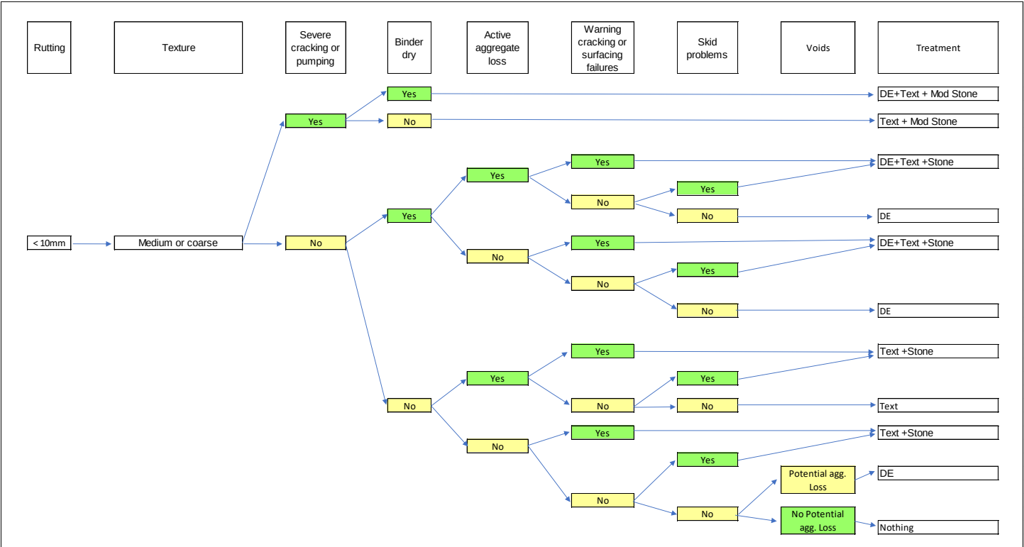
Figure D 30 Medium-to-Coarse Existing Macro Texture
