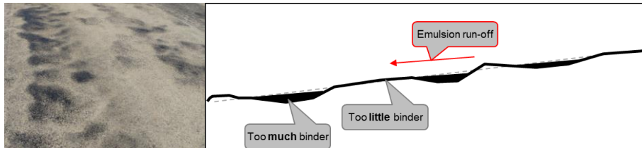
Figure C 12 Undulations Causing Ponding of Binder and Bleeding
