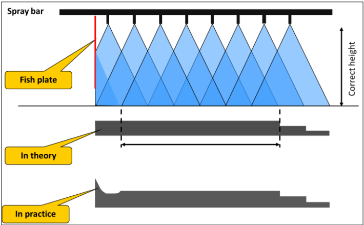
Figure F 26 Effect of Fish Plate with High Viscosity Binders
