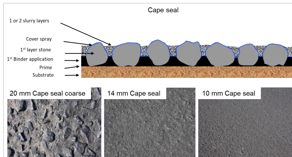
Figure A 18 Cape Seals
