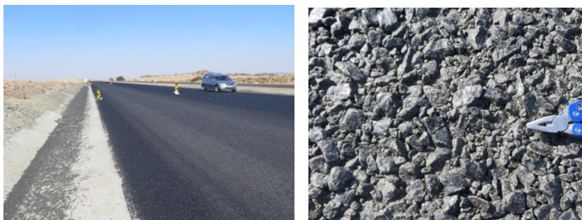
Figure H 16 Stripping of the 10mm Aggregate From a 20/10 Double Seal
