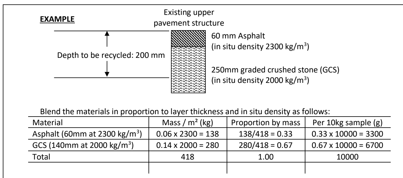
Figure 4.4 Example of Blending Exercise
