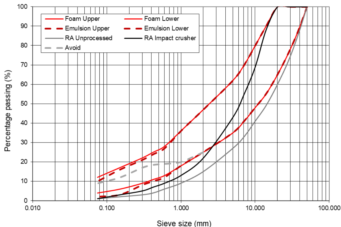
Figure 4.5 Gradients for BSM-Emulsion, BSM-Foam and RA
