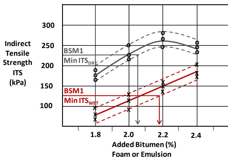
Figure 4.8 Selection of Bitumen Content from ITS DRY and ITS WET
