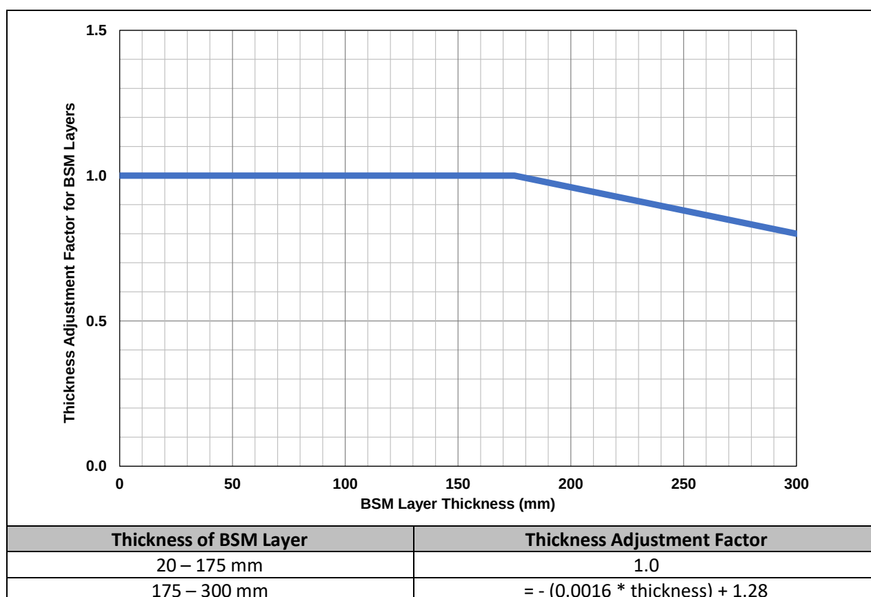
Figure C.6 Thickness Adjustment Factor for BSM Layers
